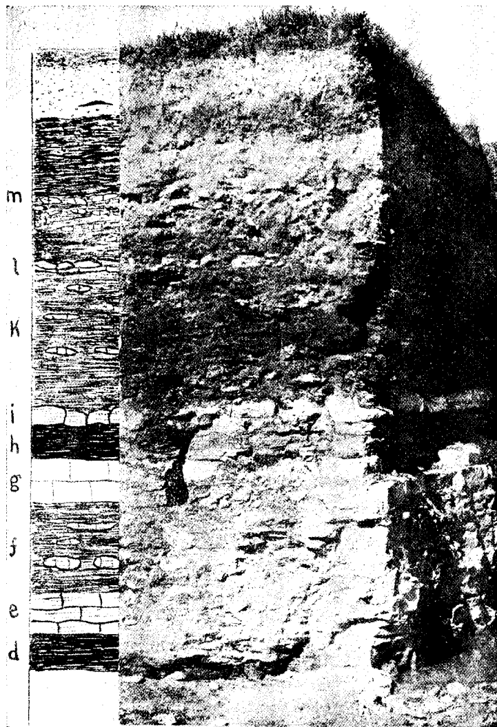
Text fig. 5. Kuckersite quarry of Järve. d — Brown kuckersite, 0.23 m.; e — Grey-brown marly-limestone containing kuckersite, 0.22 m.; f — Light-brown kuckersite with marly-limestone concretions, 0.55 m.; g — Grey-blue compact limestone „Building Limestone“, 0.26 m.; h — Light-brown kuckersite, 0.19 m.; i — Marly-limestone, containing kuckersite, 0.1 m.; k — Brown kuckersite with limestone concretions, 0.84 m.; l — Marly-limestone, often sandy, containing kuckersite, 0.06 m.; m — Dark-brown brittle kuckersite with limestone concretions in the lower portion and sand in the upper part, 0.85 m. The „Brittle kuckersite“ is overlain by boulder-clay and sand, which in the Northern portion of the quarry is stratified, 0.4 m. Photogr. by Parikas.
