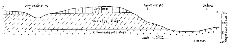
Text fig. 2. Section: Sompä—Ontika.
